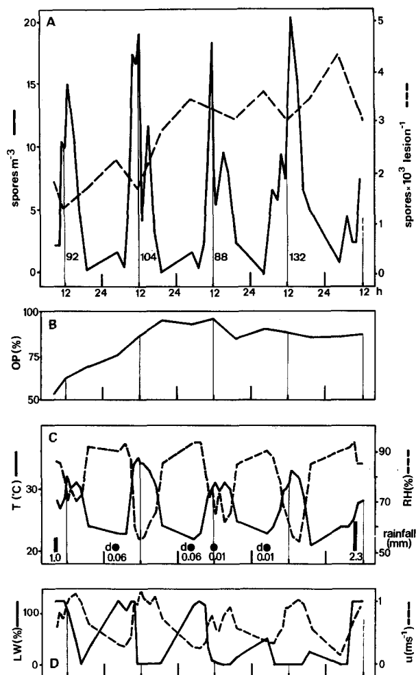
Fig. 2. Aerial dispersal of Puccinia arachidis . Diurnal periodicity of rust and weather variables in plot 1. Time is expressed in hours (horizontal axes).
