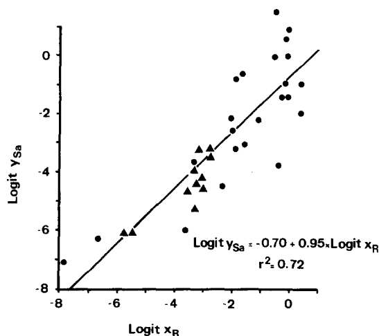
Fig. 1. Aerial dispersal of Puccinia arachidis . Spore content of the air (vertical axis) as related to rust intensity of the crop (horizontal axis).
