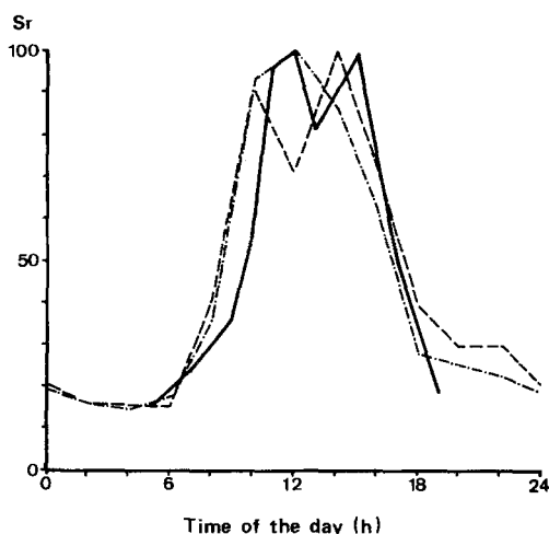
Fig. 3. Aerial dispersal of Puccinia arachidis . Diurnal periodicity of the urediniospore count of the air. S_r represents the observed spore density relative to weighted mean peak value, in percent. — Plot 1 (see text): weighted means of four days representing dry weather conditions; ---- Mallaiah and Rao (1982): variation in one rainy season; - · - · - Mallaiah and Rao (1982): mean values for three cropping seasons.
